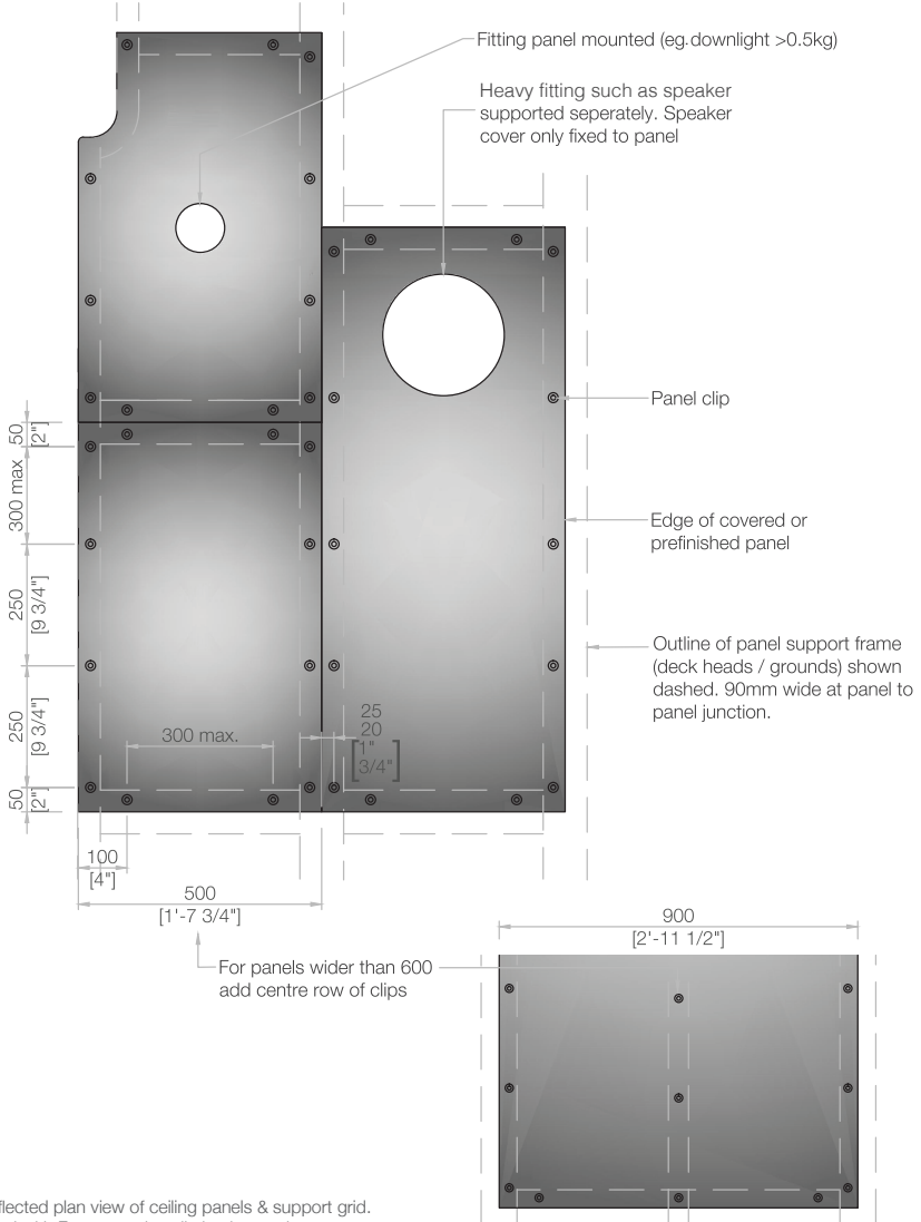
Reflected plan view of ceiling panels & support grid. Read with Fastmount installation instructions.
